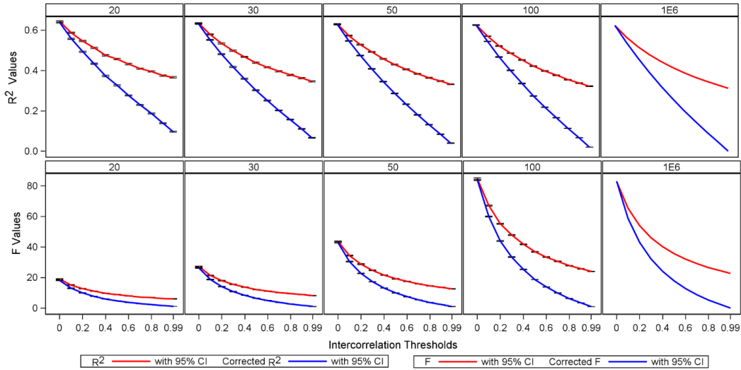
Figure 7. R^2 and Corrected R^2 , F and Corrected F ; mean values of R^2 (Red) and Corrected R^2 (Blue) and F (Red) and Corrected F (Blue) with 95% confidence intervals are provided across increasing sample sizes ( n = 20, 30, 50, 100 ) and thresholds of intercorrelation ( r_{12} = 0.00, 0.10, 0.20, 0.30, 0.40, 0.50, 0.60, 0.70, 0.80, 0.90, 0.99 ) for both; for reference, population parameter values are provided at the far right and are denoted as having a size of one million; note that the population of F and Corrected F are not to scale nor do they exist in reality; they are provided for comparison of behavior, not value
