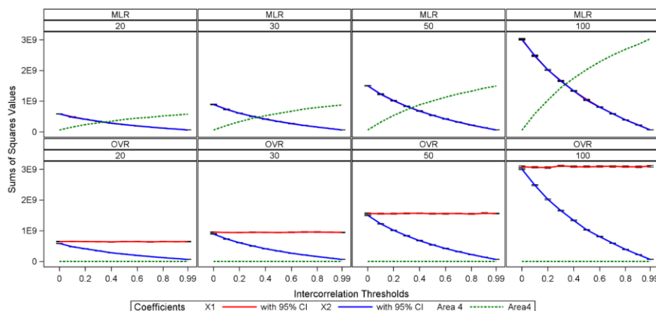
Figure 5. Predictor sums of squares for samples; mean values of X_1 (red), X_2 (blue), and Area 4 (green) with 95% confidence intervals are provided across increasing sample sizes ( n = 20, 30, 50, 100 ) and thresholds of intercorrelation ( r_{12} = 0.00, 0.10, 0.20, 0.30, 0.40, 0.50, 0.60, 0.70, 0.80, 0.90, 0.99 ) for both; values are presented by model: MLR (top) and OVR (bottom); Note that Area 4 is part of X_1 (red) for OVR but is shown as a green line for comparison with MLR
