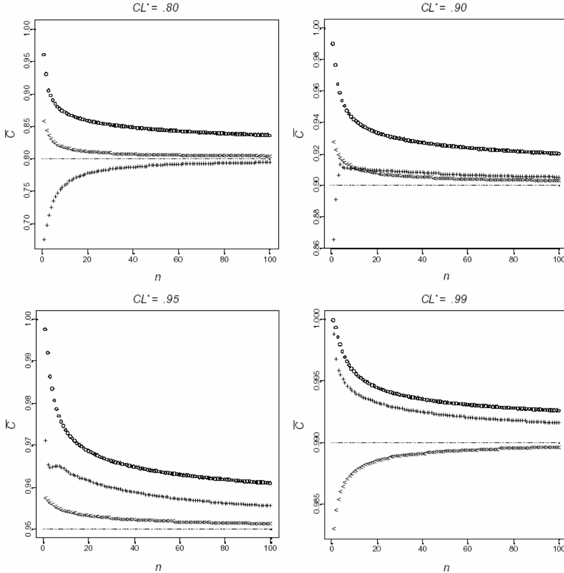
Figure 2. Average Coverage Probabilities of Three Approximate Methods. The scatter is of the average coverage probabilities of three approximate methods when p is uniformly distributed for sample sizes of from 1 to 100 with nominal confidence levels of .80, .90, .95, and .99. The optimized interval method is indicated by a “o”, the adjusted Wald method by a “+”, and the score method by a “<”. The horizontal dotted line is at the nominal confidence level. The optimized interval method’s average coverage probability tends to be further away from the nominal than the other two methods for all four nominal confidence levels and is always higher than the nominal. The average coverage probabilities of the other two methods tend to be closer to, and sometimes below, the nominal level.
