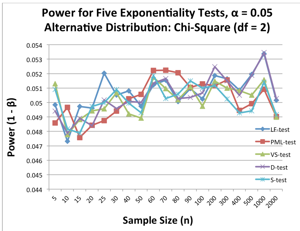
Figure 8. Power for Alternative Distribution: Chi-Square (2)
